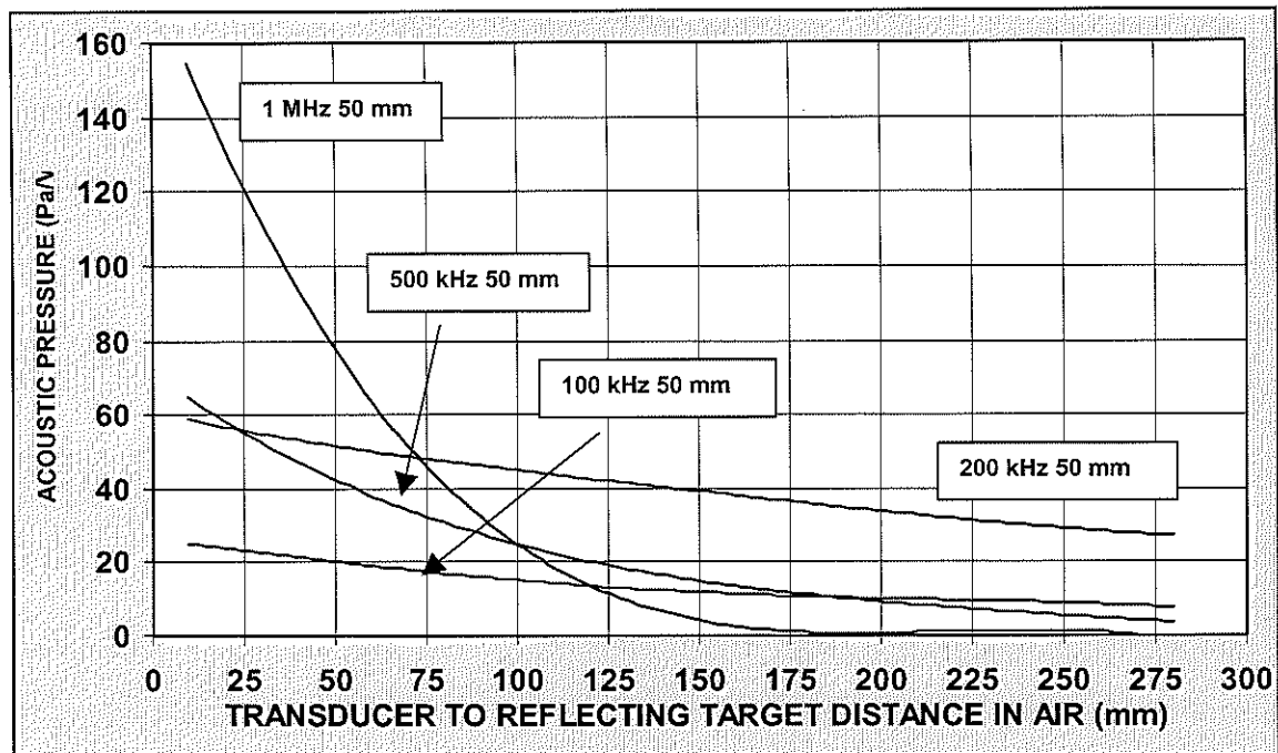
Fig. 1. Acoustic pressure of selected NCU transducers, identified by frequency and active area diameters, as a function of transducer to reflecting target distance in ambient air. Transducers used as reference were calibrated by Laser interferometric technique at Laboratoire de Mécanique Physique, Université Bordeaux, France.
