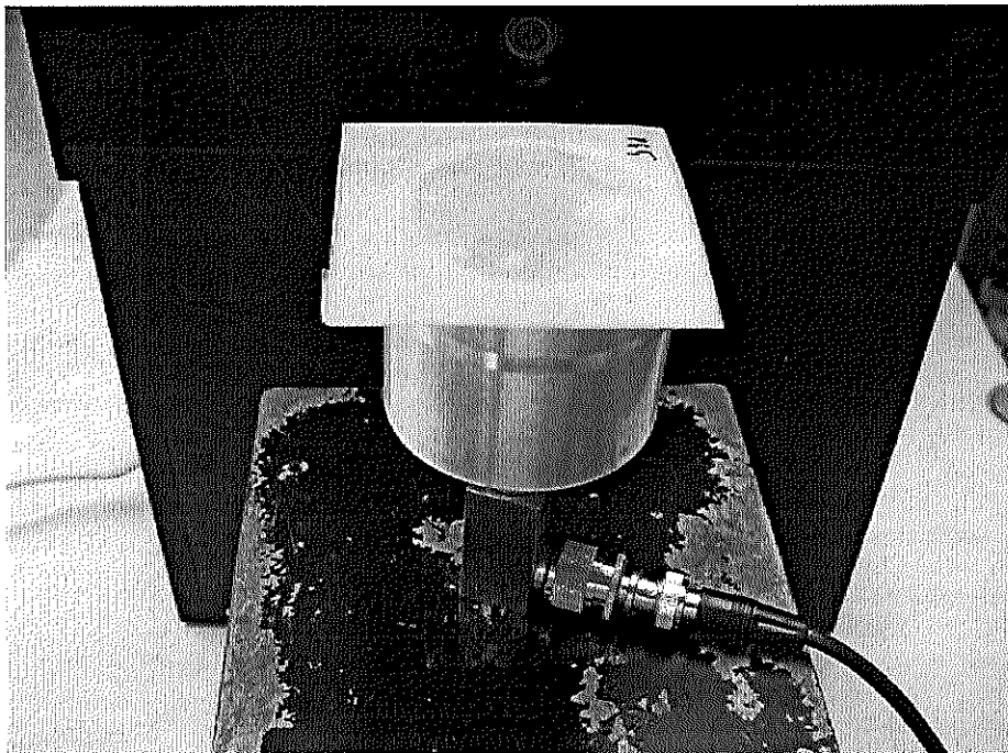
Figure 2. Non-Contact Ultrasound transducer with an envelope containing spores of Bacillus thuringiensis in treatment position. The space between the envelope and the transducer is approximately 3 mm. Note that there is no medium present to provide any contact between the envelope and the transducer.
